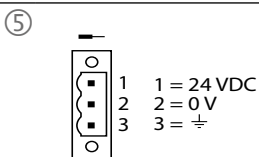
Voltage supply
