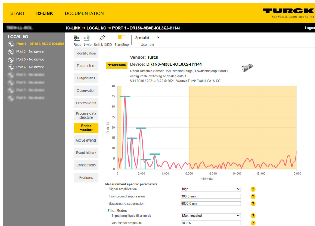
Fig. 93: Radar monitor
