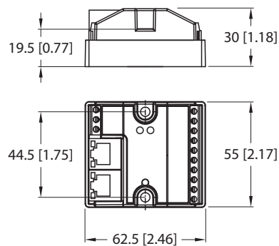
Fig. 1: Dimensions FEN20-4IOL
