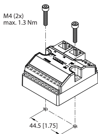
Fig. 3: Mounting the device onto a mounting plate
