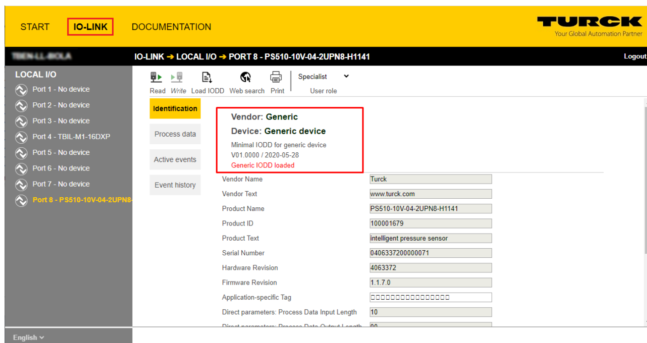
Fig. 68: IO-Link device with generic IODD
