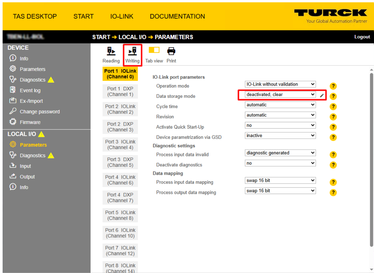
Fig. 82: TAS: deleting the data storage memory via parameters
