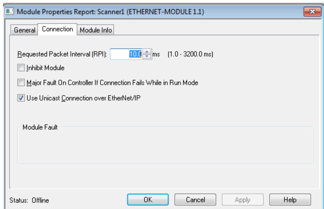
Fig. 49: Setting the connection parameters
