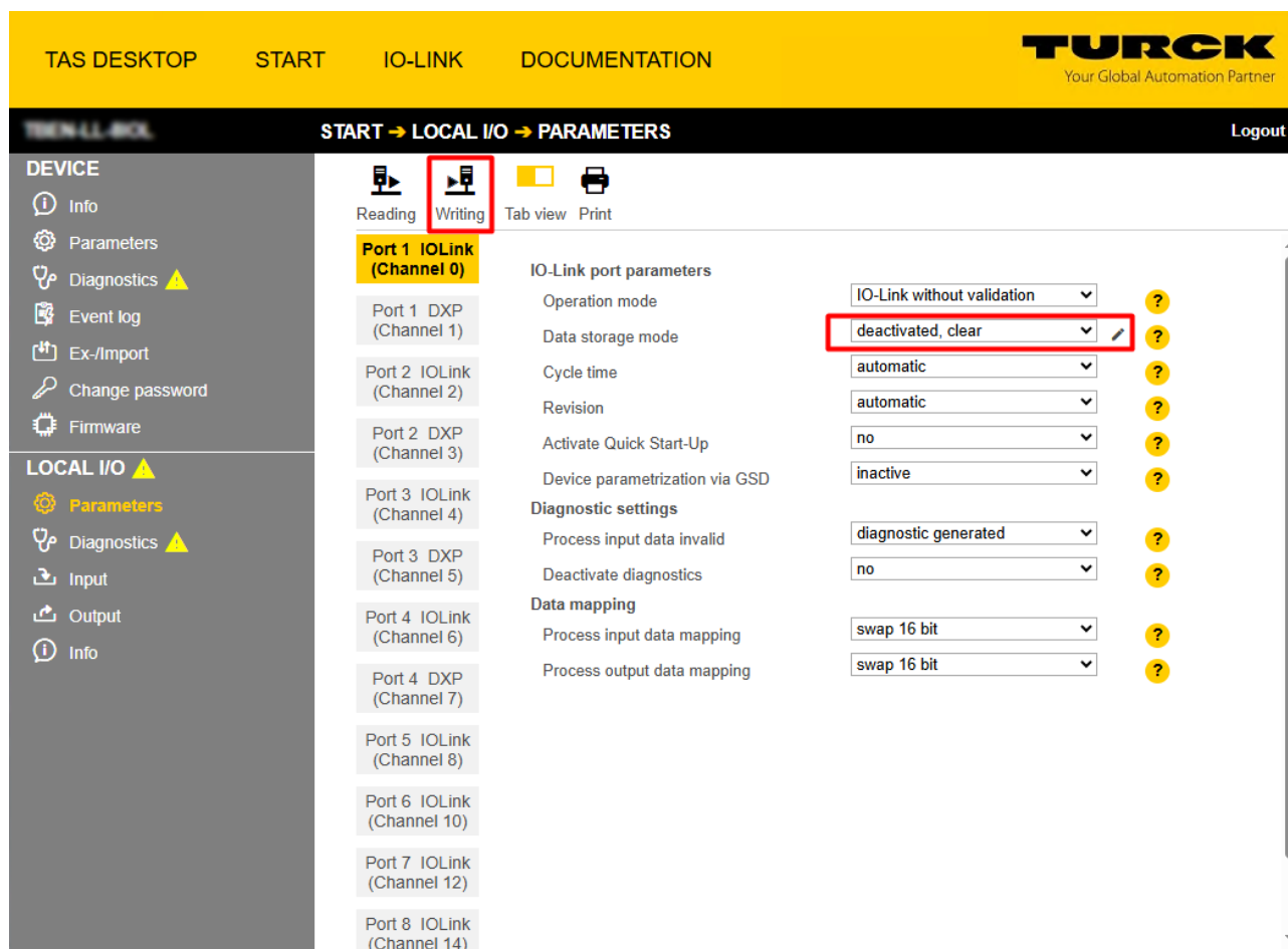
Fig. 80: TAS – deactivate data storage
