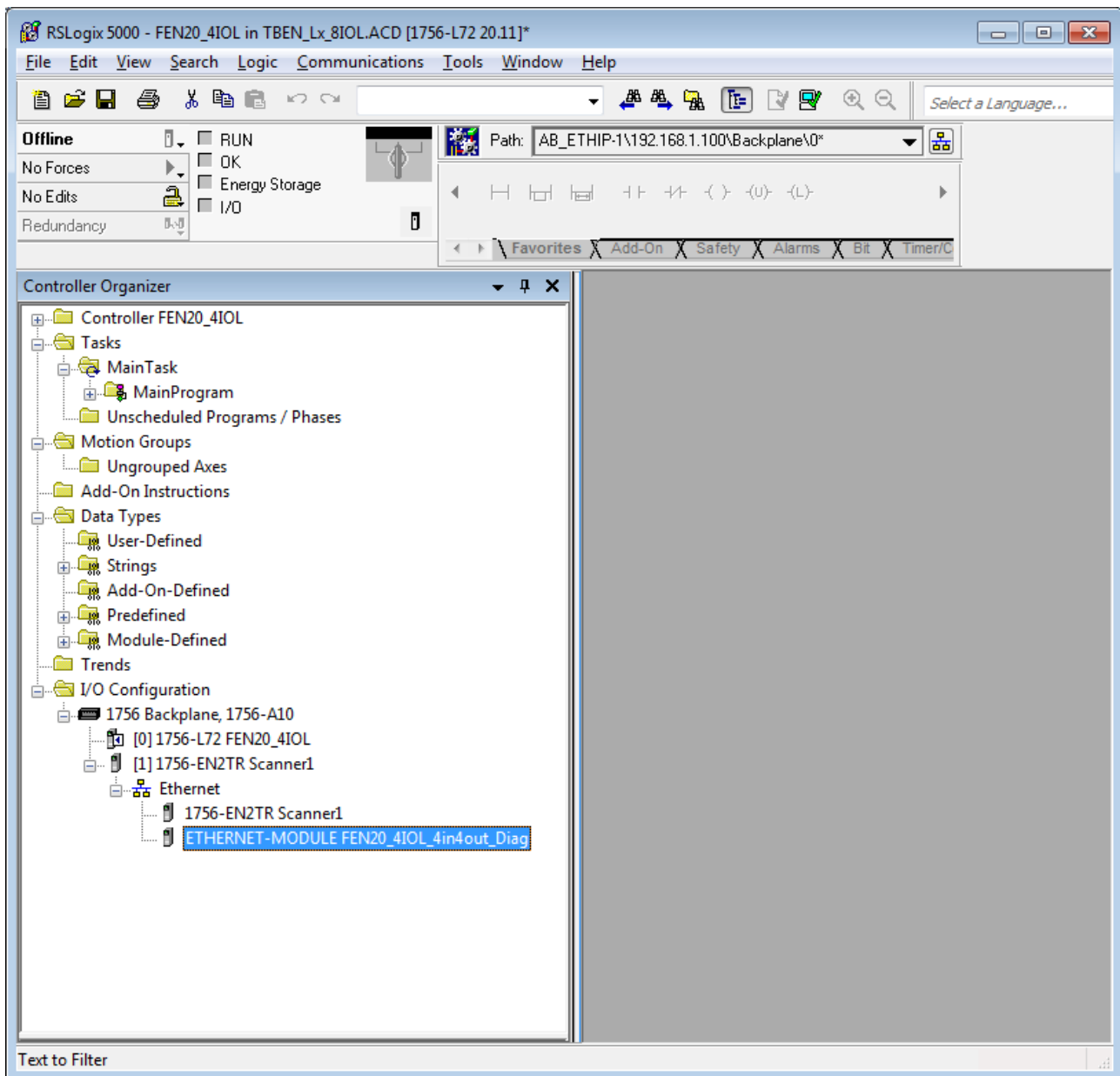
Fig. 47: RSLogix – predefined configurations of FEN20-4IOL in new project
