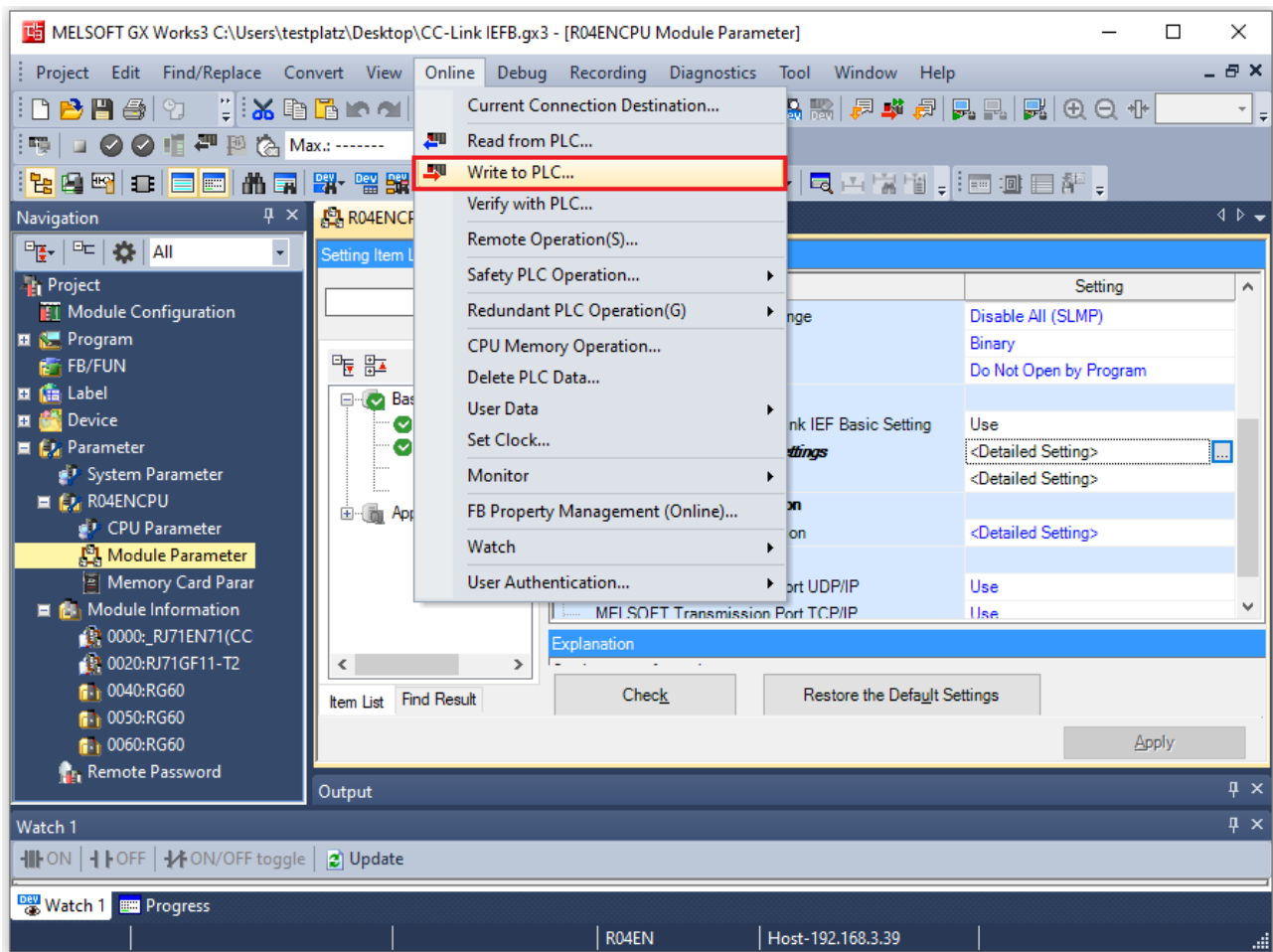
Fig. 64: GX Works3: Writing the configuration to the PLC
