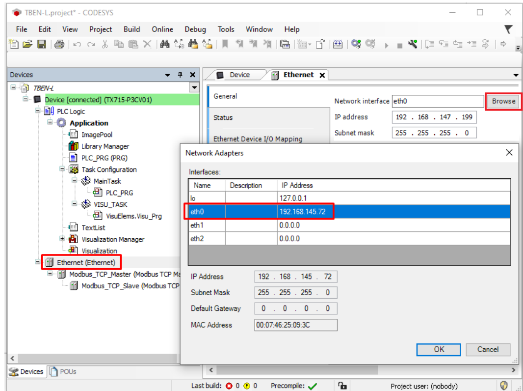
Fig. 39: Selecting the interface
