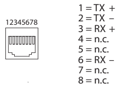
Fig. 7: Ethernet connectors – pin assignment P1 and P2
