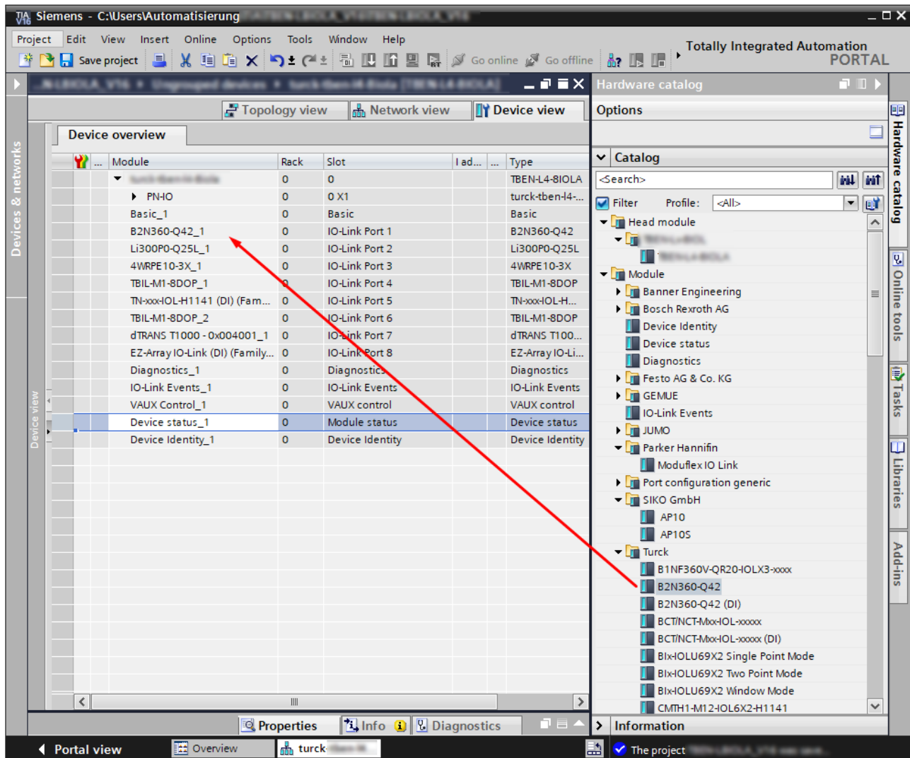
Fig. 71: Example: TIA Portal, IO-Link device in hardware catalog (SIDI)
