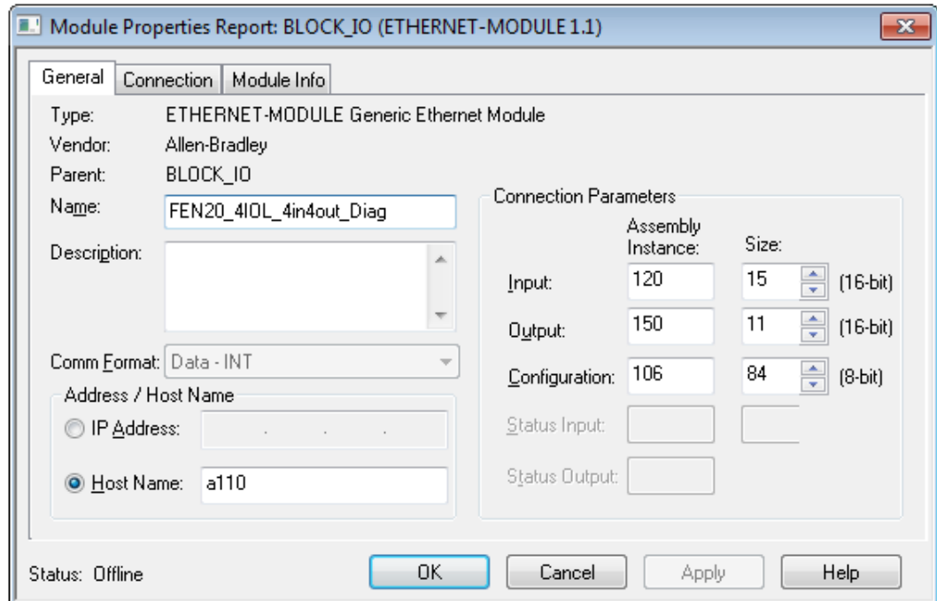
Fig. 48: Setting module name and IP address
