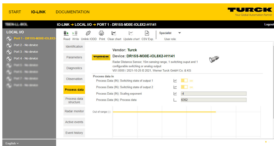
Fig. 90: Process data of an IO-Link device
