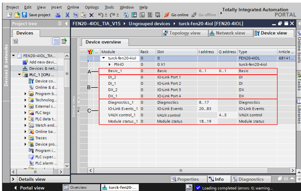
Fig. 17: FEN20-4IOL – slot overview in in TIA-Portal
