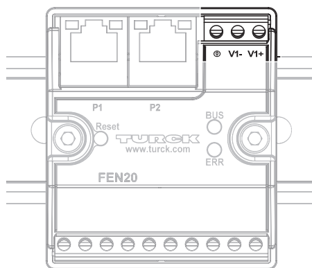
Fig. 5: Fieldbus and I/O level shielding
