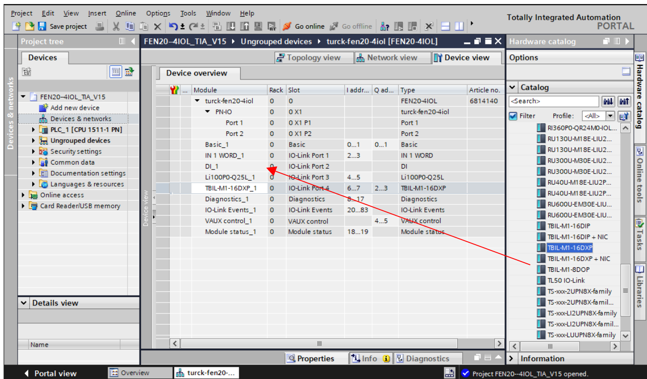
Fig. 23: TIA-Portal – configuring device slots
