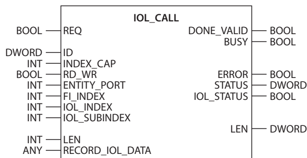
Fig. 18: IOL_CALL in accordance with IO-Link specification
