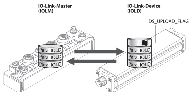
Fig. 83: Data storage mode – general principle, Para. IOLD = parameters of the IO-Link device
