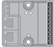
Fig. 10: Terminal screw connector for connecting IO-Link devices and digital sensors and actuators
