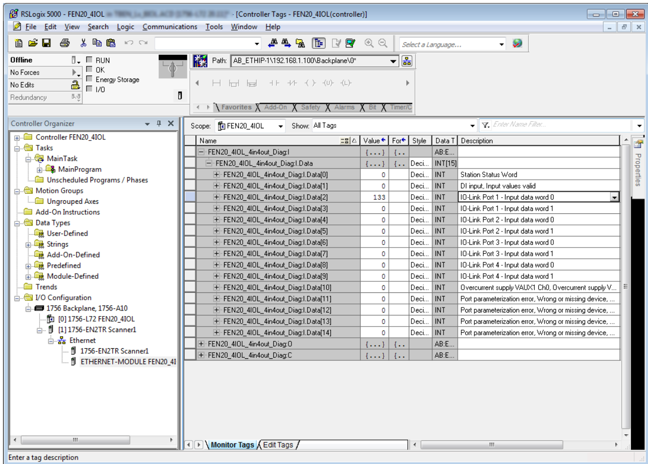
Fig. 53: Controller Tags in the project tree
