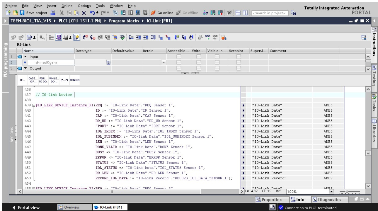
Fig. 26: Example call of Siemens FB "IO_LINK_DEVICE"
