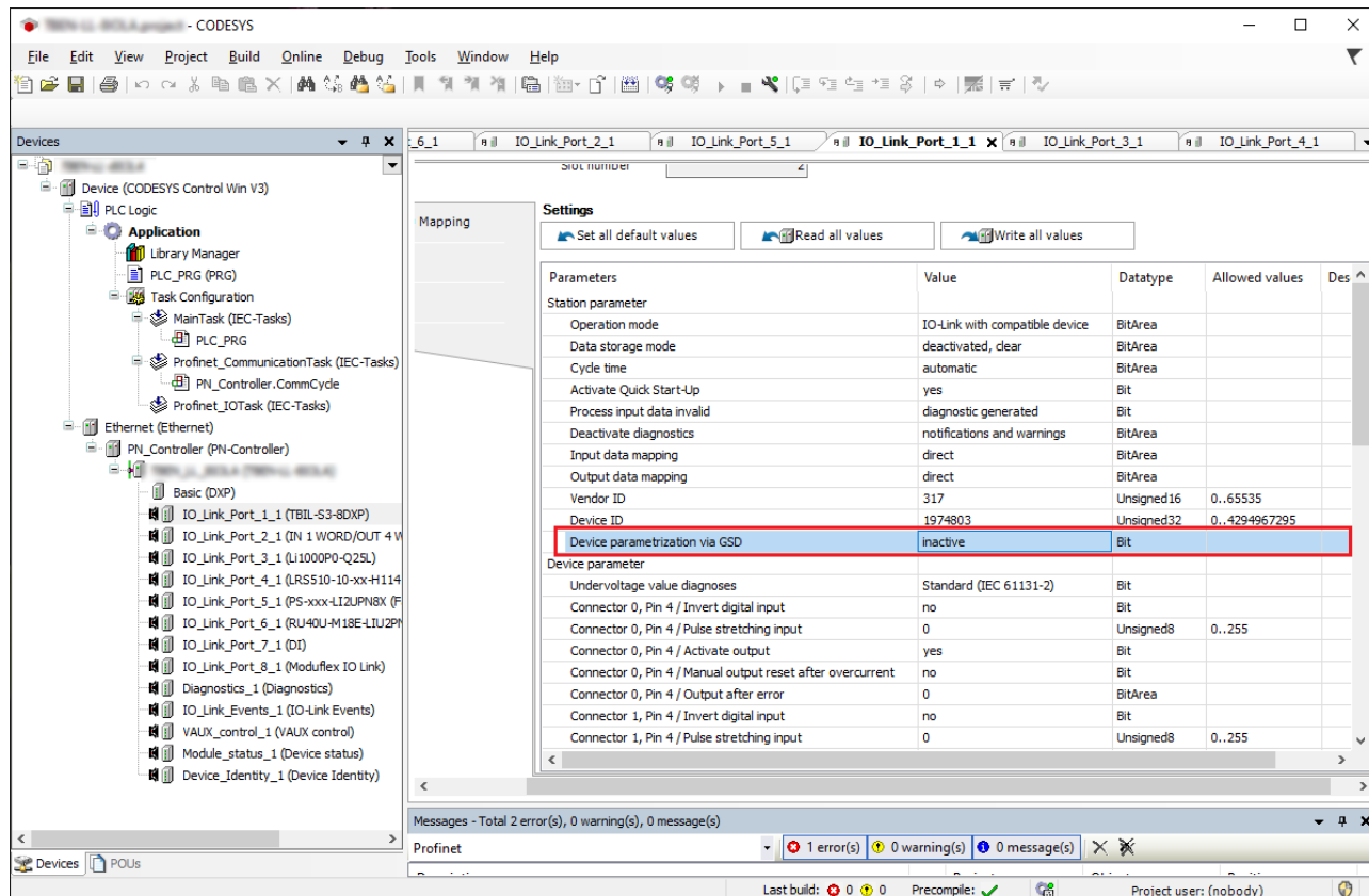
Fig. 74: PROFINET engineering (CODESYS); Device parameterization via GSD inactive
