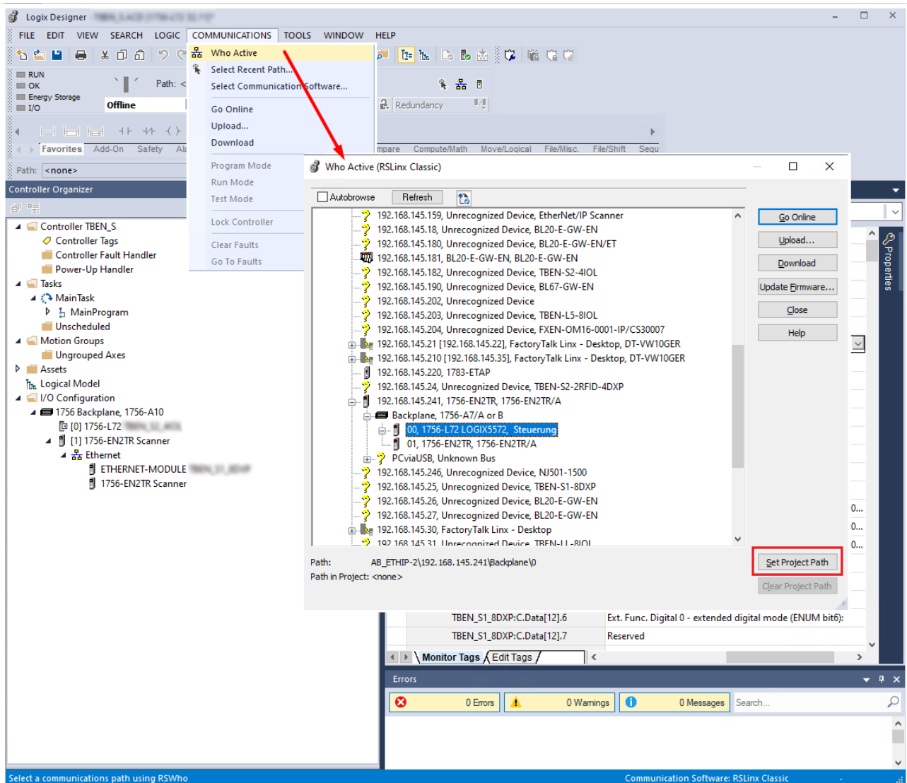
Fig. 51: Setting the communication path
