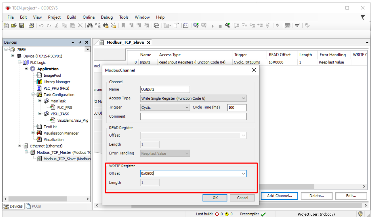
Fig. 42: Defining the output data register
