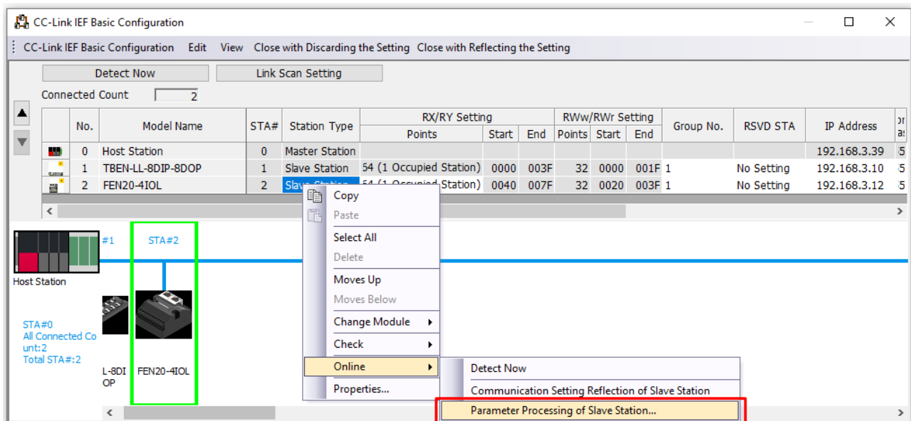
Fig. 59: GX Works3: Opening parameterization
