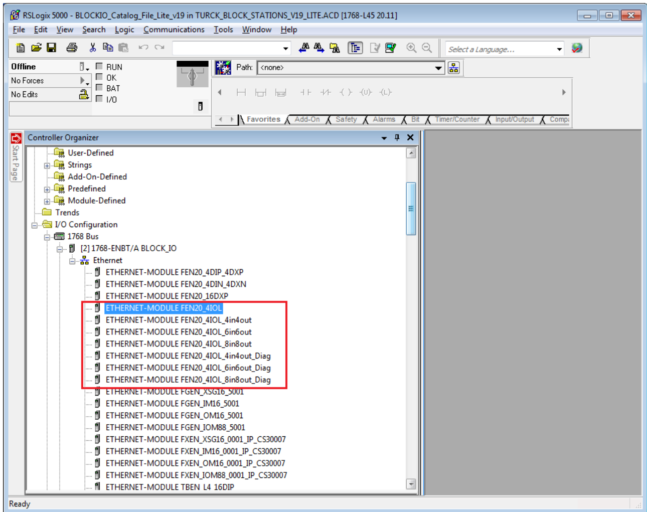
Fig. 46: RSLogix – Copying the device entry from catalog file
