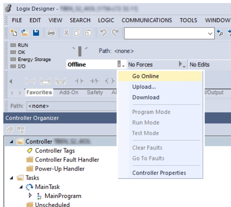
Fig. 52: Going online with the device
