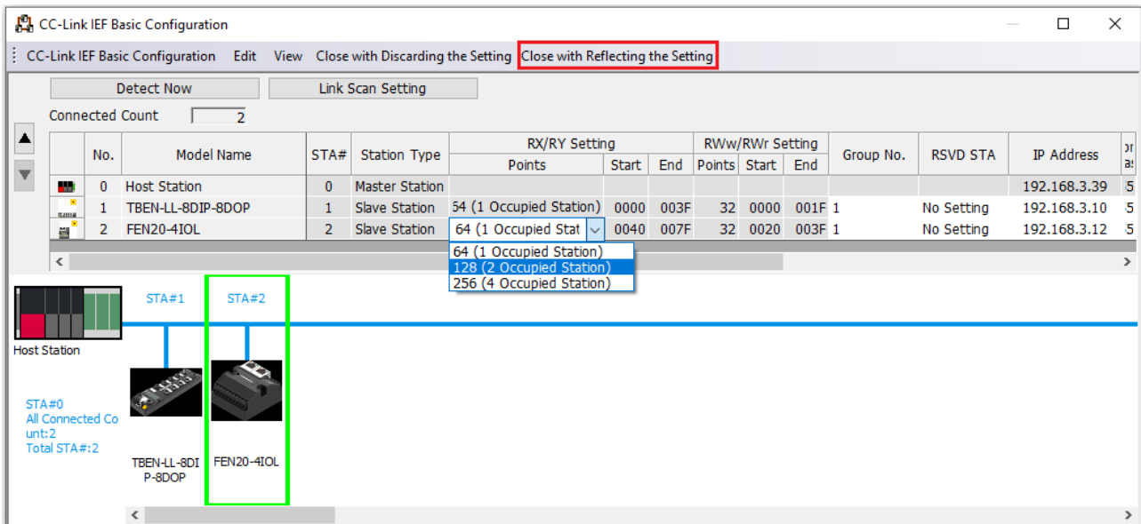
Fig. 61: GX Works3: Storing the network structure
