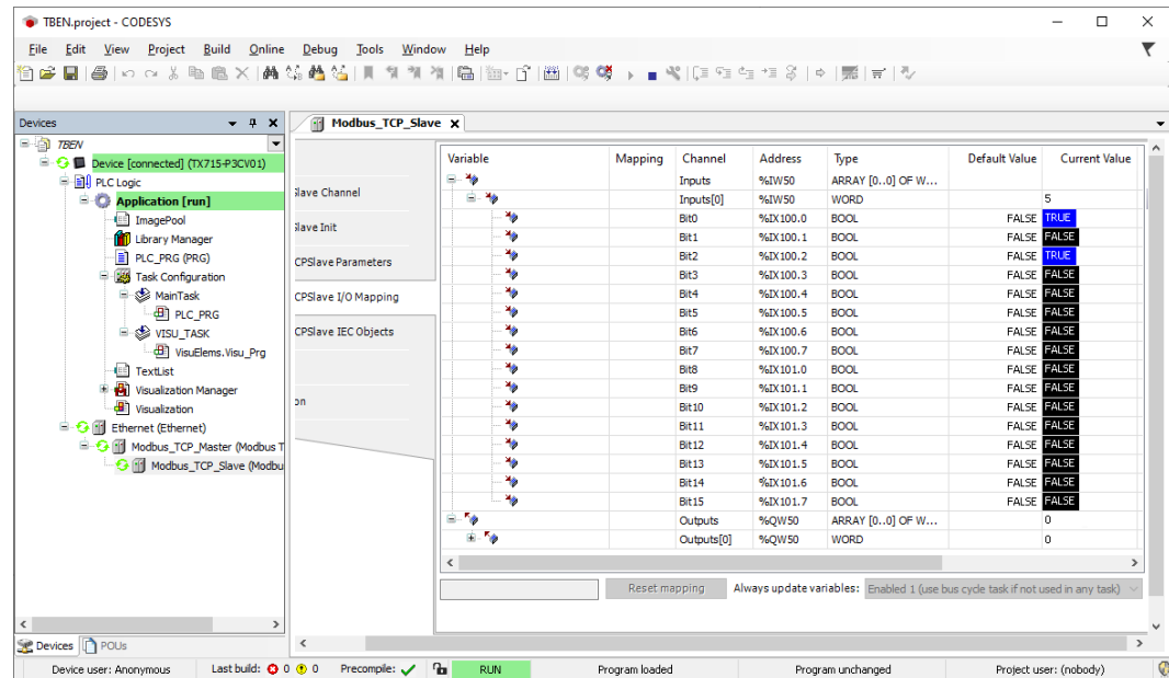
Fig. 45: Process data
