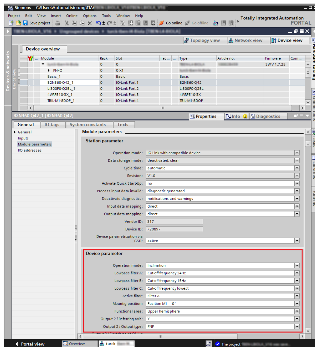
Fig. 73: Example: TIA Portal, IO-Link device parameters via GSDML
