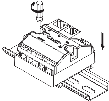
Fig. 4: Mounting the device with mounting adapter on DIN rail
