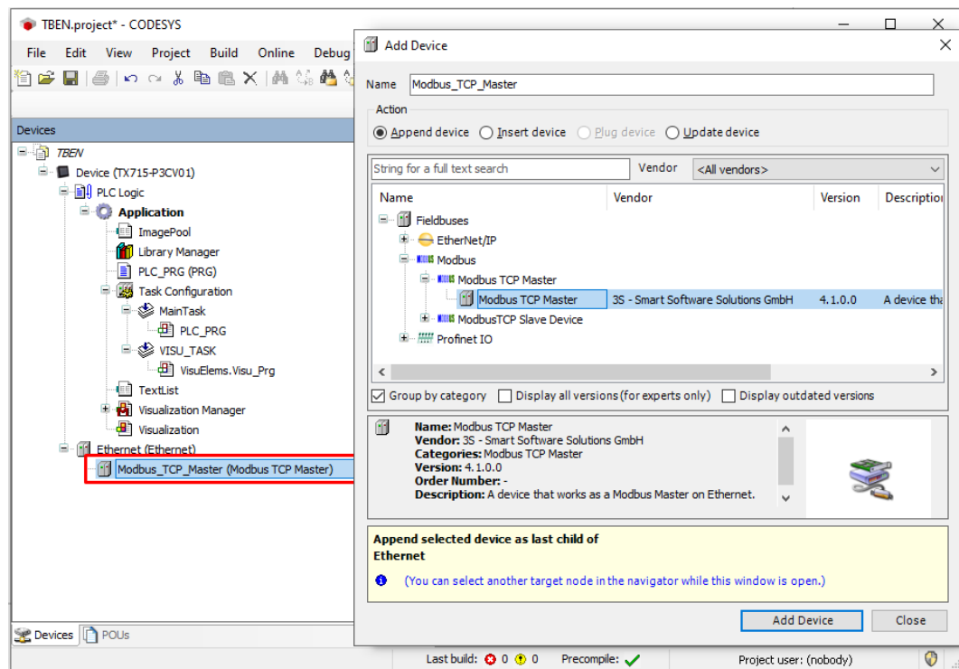
Fig. 36: Adding the Modbus TCP Master
