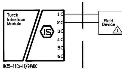
IM35-11Ex-Hi/24VDC
