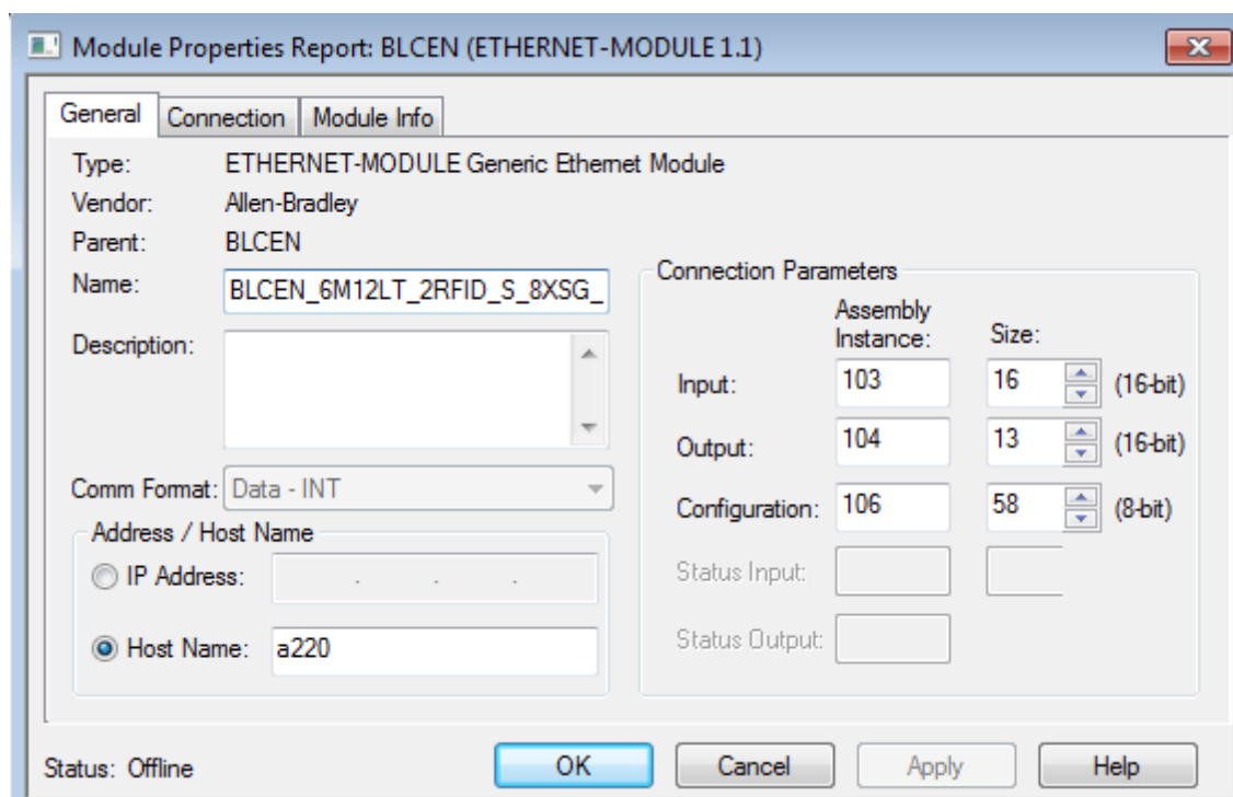
Figure 1: Generic Ethernet Module configuration page
