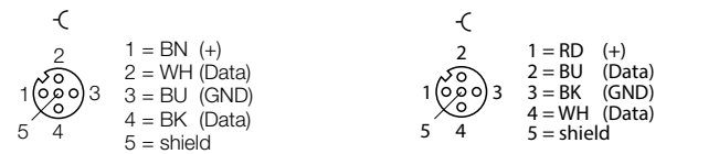
RFID channels (C0...C3) – Connectors .../ S2501
