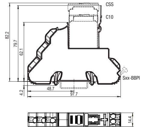
fig. 2. Dimension (mm)
