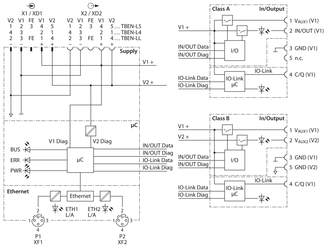
Fig. 3: Block diagram
