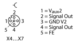
M12 × 1 Output
