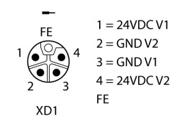
M12 power supply, L-coded
