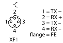
M12 × 1 Ethernet
