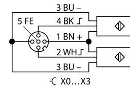
M12 × 1 Output
