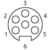
Connector B
