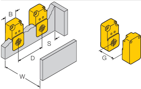
Mounting instructions/Description
