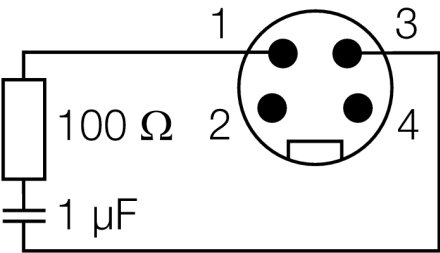
Wiring Diagram
