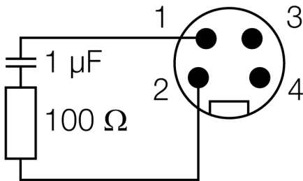
Wiring Diagram
