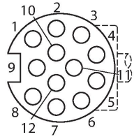
Connector A
