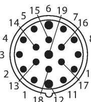
Homerun connector
