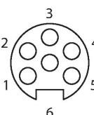
Connector B
