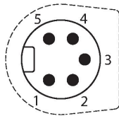
Connector A
