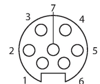
Connector B
