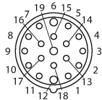
Connector A
