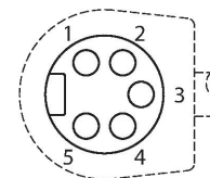
Connector A
