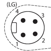
Connector A
