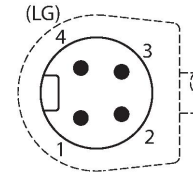
Connector A
