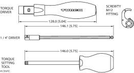
TORQUE-WRENCH-SET-M12-LEGACY
