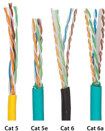
As the speed increases, so does the twisting of pairs and shielding
